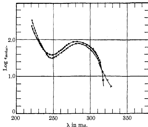
Fig. 2.—Curve 1 (crosses), desoxysarsasapogenoic acid ( C_{27}H_{42}O_4 \cdot H_2O ) in absolute alcohol; curve 2 (circles), sarsasapogenoic acid acetate in absolute alcohol.
