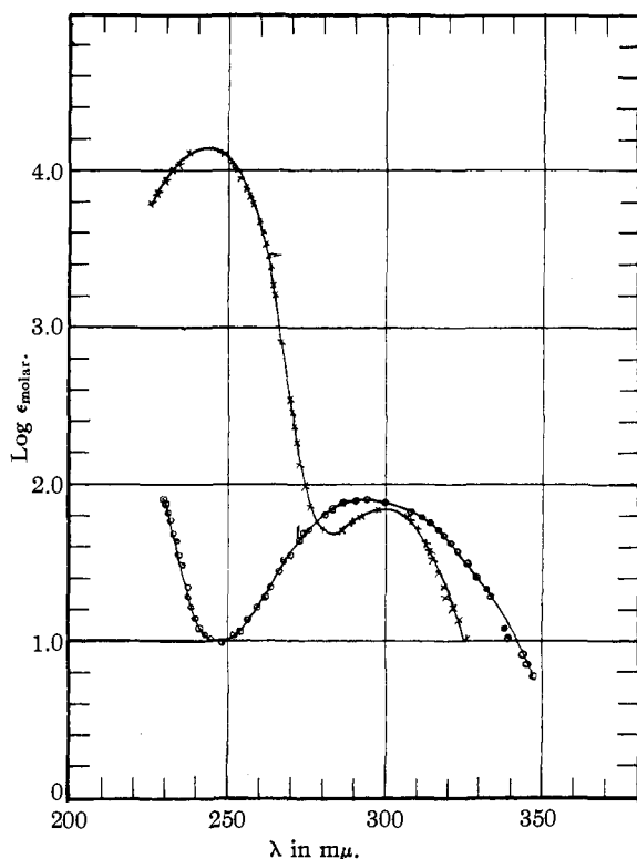
Fig. 1.—Curve 1 (crosses), anhydrosarsasapogenoic acid methyl ester acetate in absolute alcohol; curve 2 (circles), dimethyl ester of dibasic acid C_{27}H_{40}O_7 in absolute alcohol.
